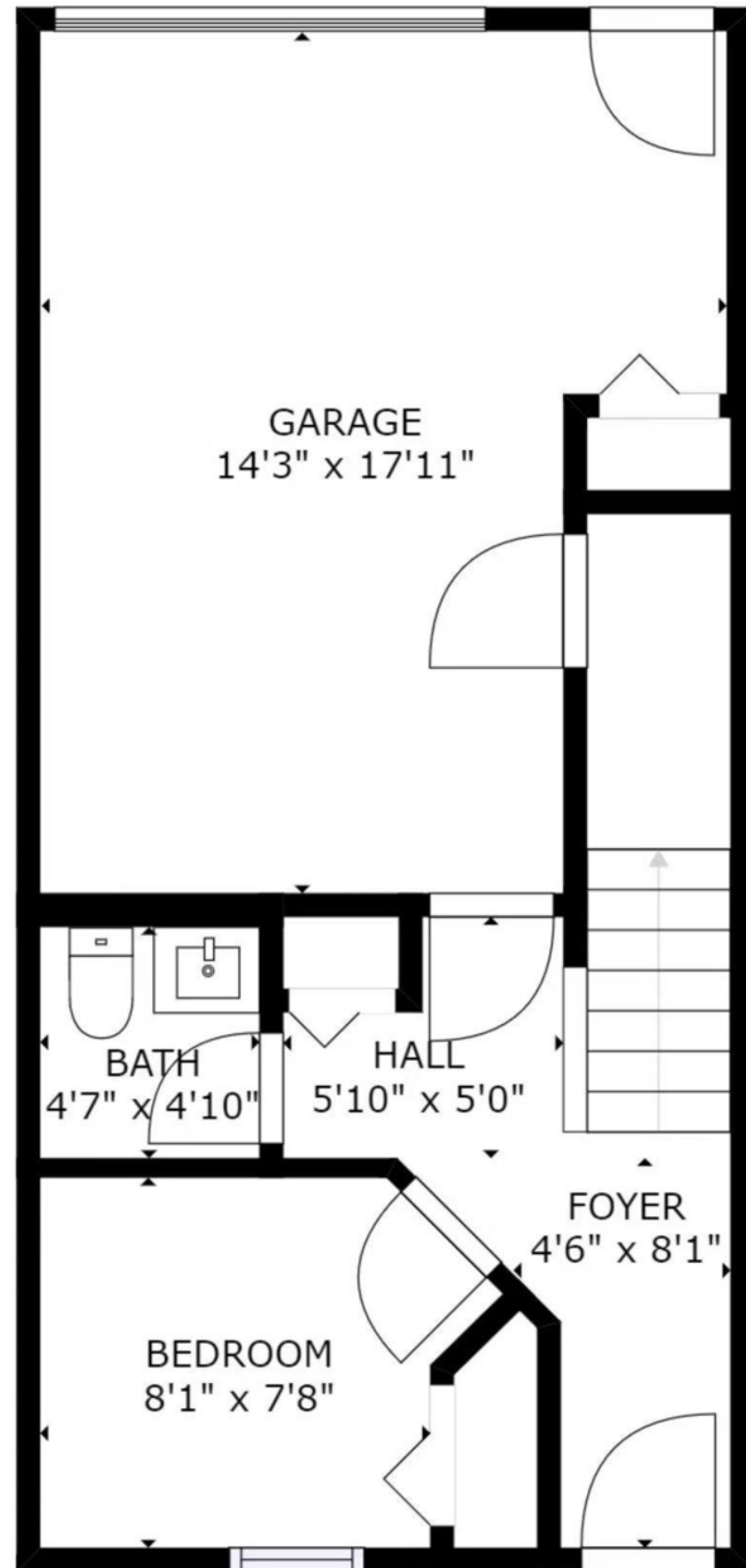
FLOOR 1
